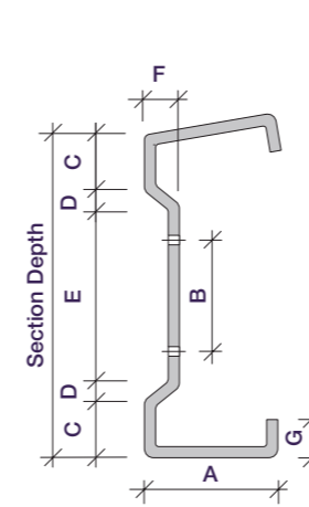
200 Eaves Beam Series
