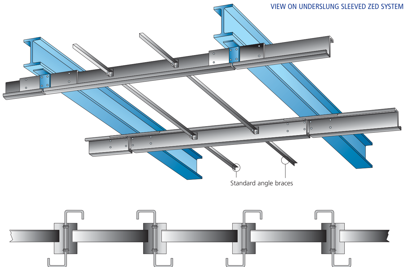
TYPICAL SECTION THROUGH ZEDS SHOWING ALTERNATE DIRECTIONS OF SECTIONS
