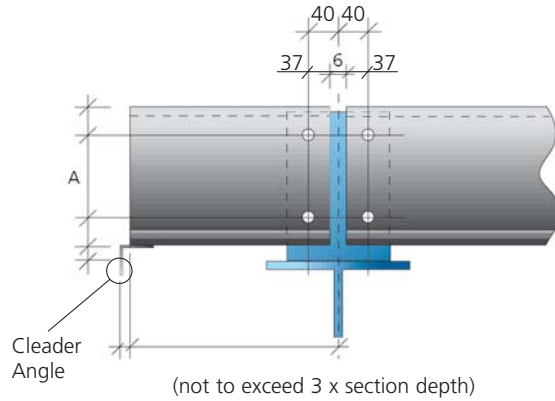
ALTERNATIVE GABLE PURLIN DETAIL (or can use a sleeve at extendable gable)
