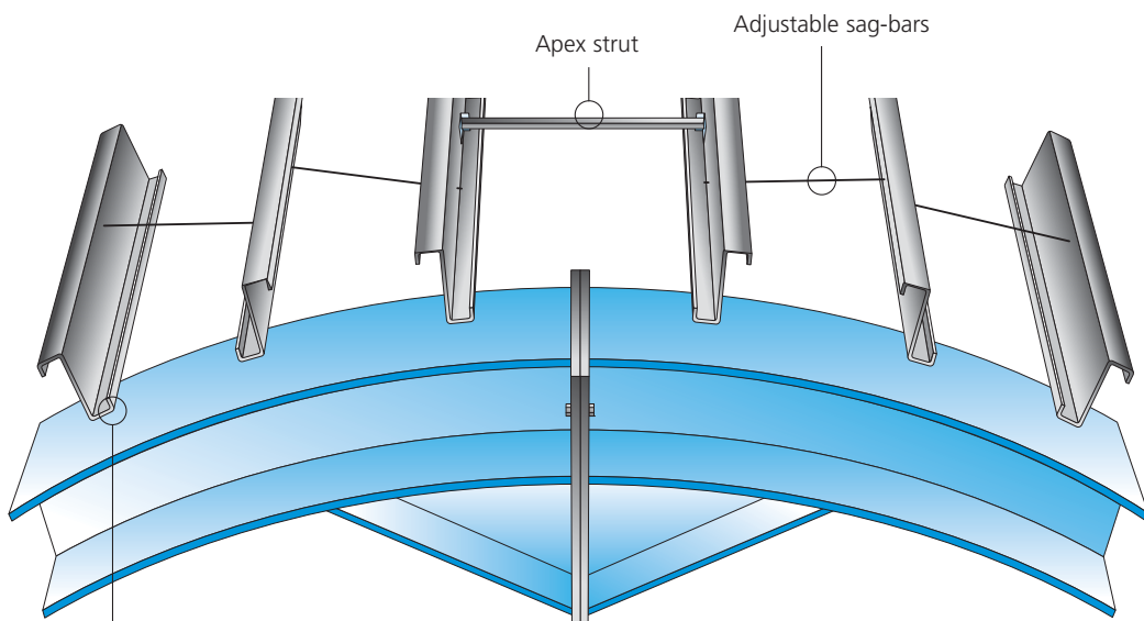
Alternative purlin directions reversed when roof tangent is less than 3°
