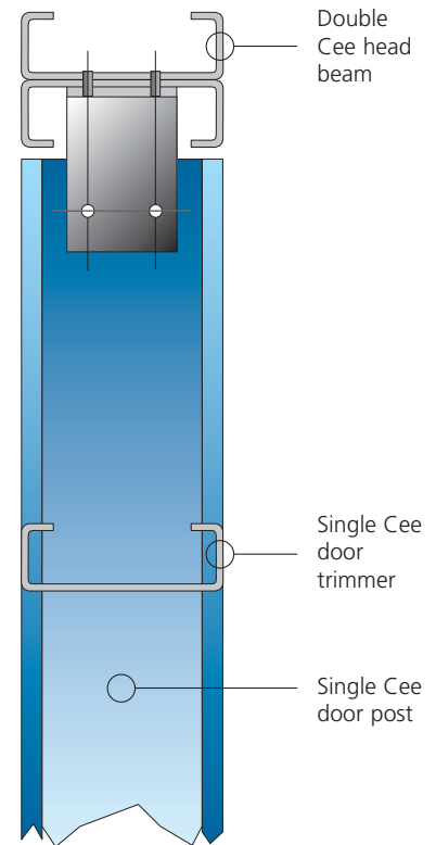
SECTION THROUGH TYPICAL OVERHEAD DOOR
