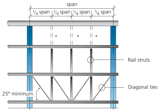
TRIPLE ROW STRUT SYSTEM
