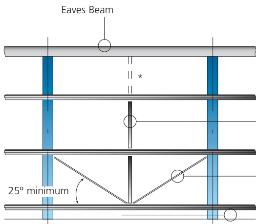
SINGLE ROW STRUT SYSTEM
