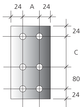
Galv steel 3mm thick 14mm dia holes
