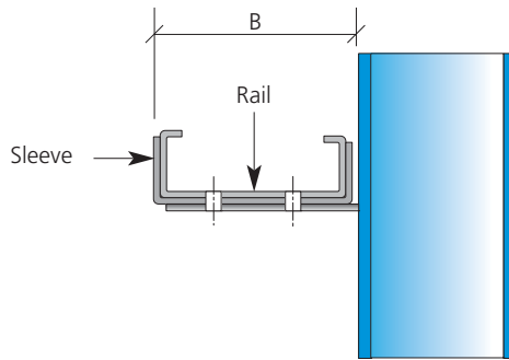
CEE RAILS
