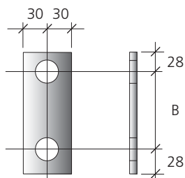
Galv 6mm thick plate 36mm dia holes
