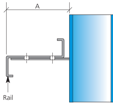
ZED RAILS
