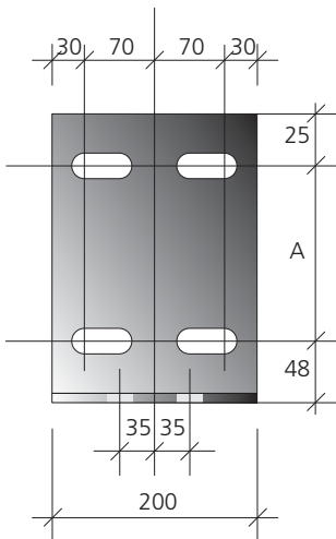
NORMAL FIRE WALL CLEATS
