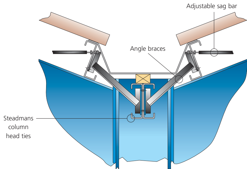
HEAD TIE DETAIL WITH GUTTER SUPPORTED BY HEAD TIES
