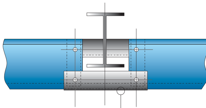
Rail closer from 45 x 70 Galv angle x 2mm thick
