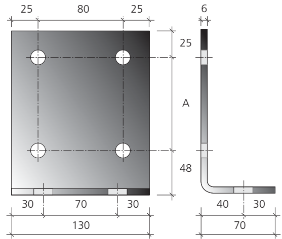
BOLT-ON CLEATS
