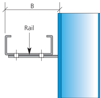
CEE RAILS
