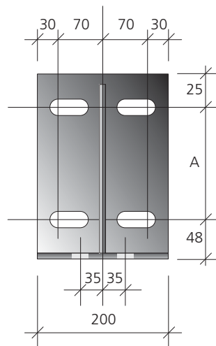
HEAVY DUTY FIRE WALL CLEATS
