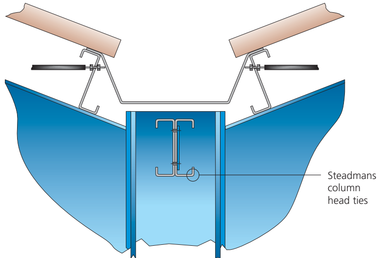
HEAD TIE DETAIL WITH NO GUTTER SUPPORT
